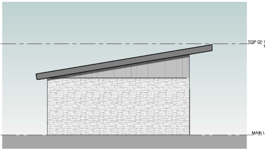
4 NORTH ELEVATION 3/16" = 1'-0"
