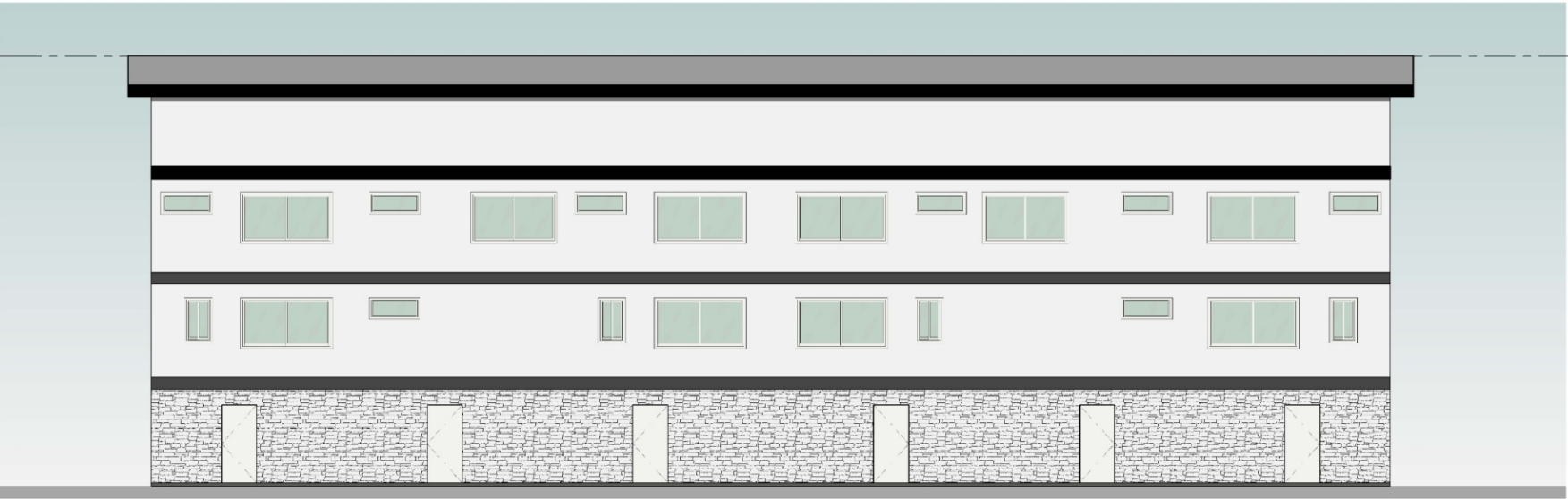
1 EAST ELEVATION 3/16" = 1'-0"
