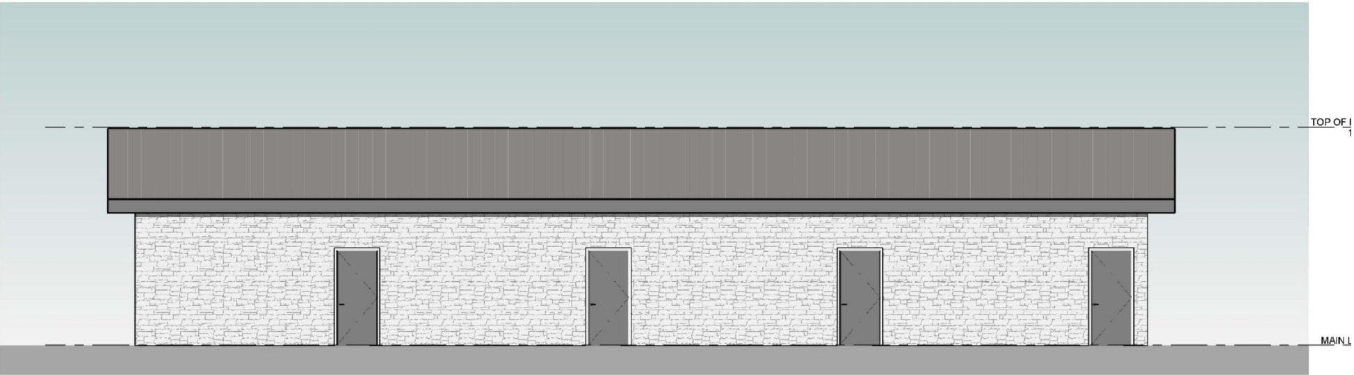
1 WEST ELEVATION 3/16" = 1'-0"
