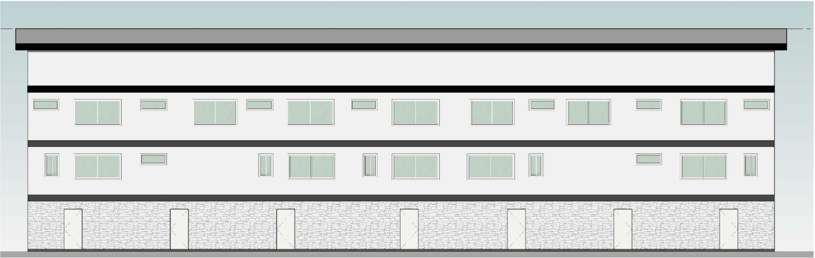
1 EAST ELEVATION 3/16" = 1'-0"
