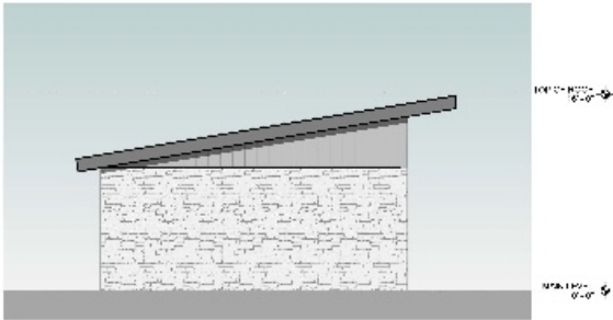
4 NORTH ELEVATION 3/16" = 1'-0"
