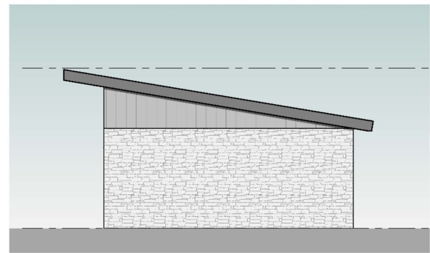
2 SOUTH ELEVATION 3/16" = 1'-0"
